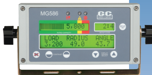
Model 586 For industrial carry-deck and truck crane applications
